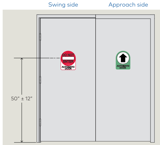
Fig. 7.5.10 Double egress, LH, two way traffic, exterior
