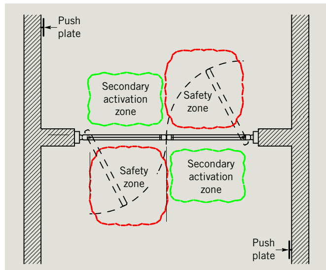
Fig. 5.1.3 Double egress, overhead presence sensors
