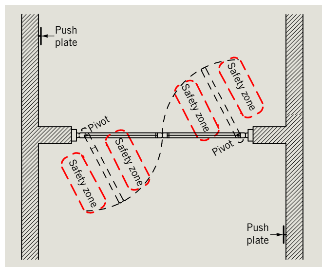
Fig. 5.1.4 Double egress, overhead presence sensors
